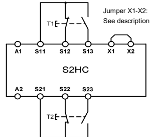
Fig. 2: Feedback loop
