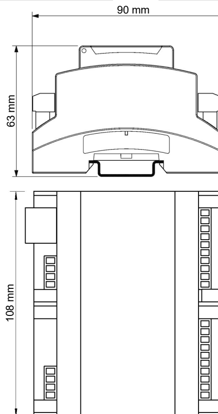
Dimensional drawing (identical measures for all controller types)
